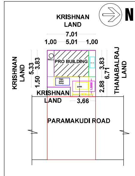
SITE PLAN & KEY PLAN
