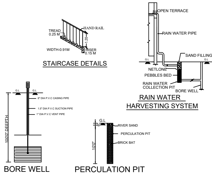
BORE WELL
