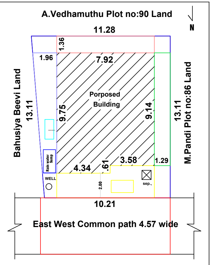
SITE PLAN CUM KEYPLAN
