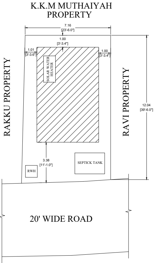
SITE PLAN
