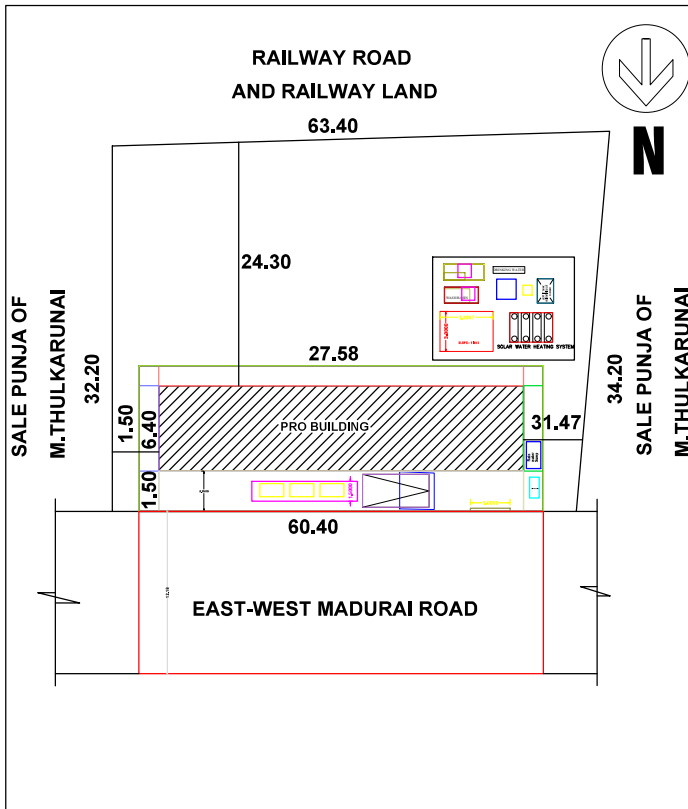
SITE PLAN & KEY PLAN
