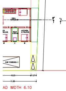
GND FLOOR PLAN
