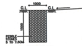
SECTION OF PEBBLE TRENCH SCALE : 1: = 100
