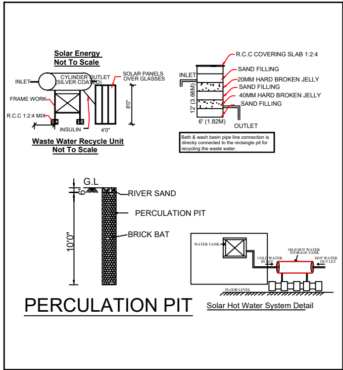
PERCUATION PIT
