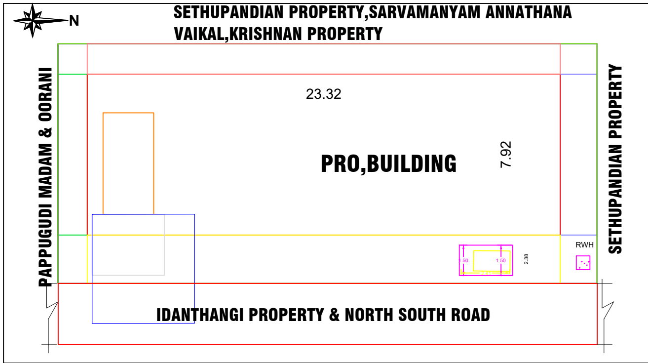
SITE PLAN
