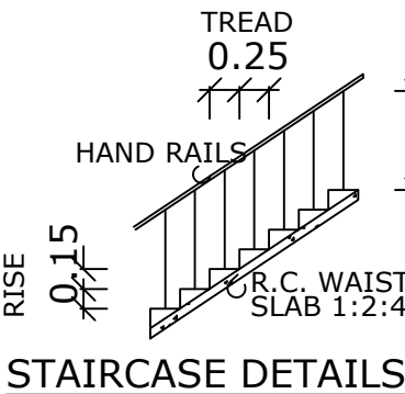
STAIRCASE DETAILS
