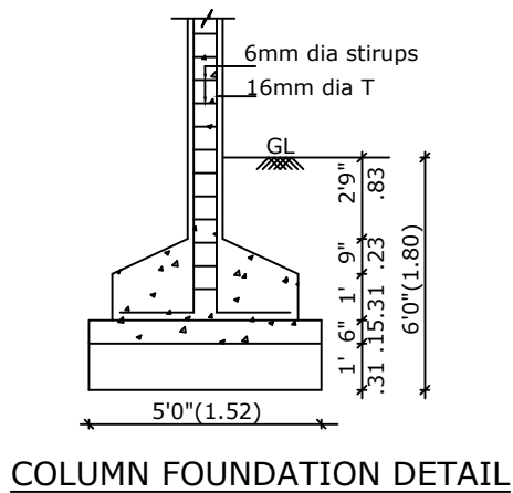
COLUMN FOUNDATION DETAIL
