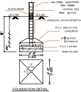
FOUNDATION DETAIL
