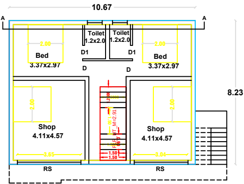
PRO. FIRST FLOOR PLAN
