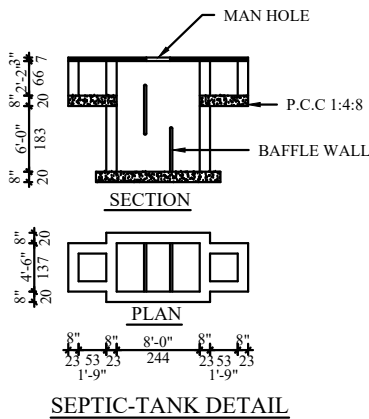
SEPTIC-TANK DETAIL
