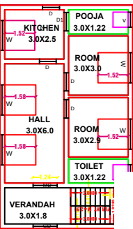
GROUND FLOOR P1
