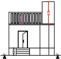
FRONT ELEVATION
