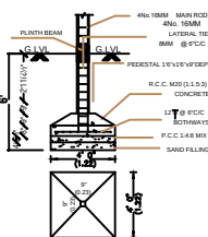
FOUNDATION DETAIL
