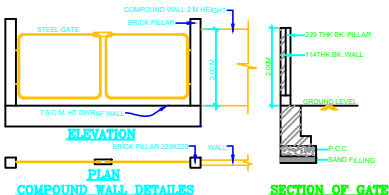
SECTION OF GATE
