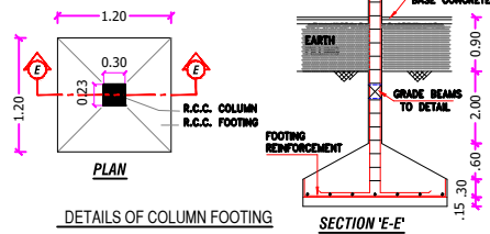
DETAILS OF COLUMN FOOTING
