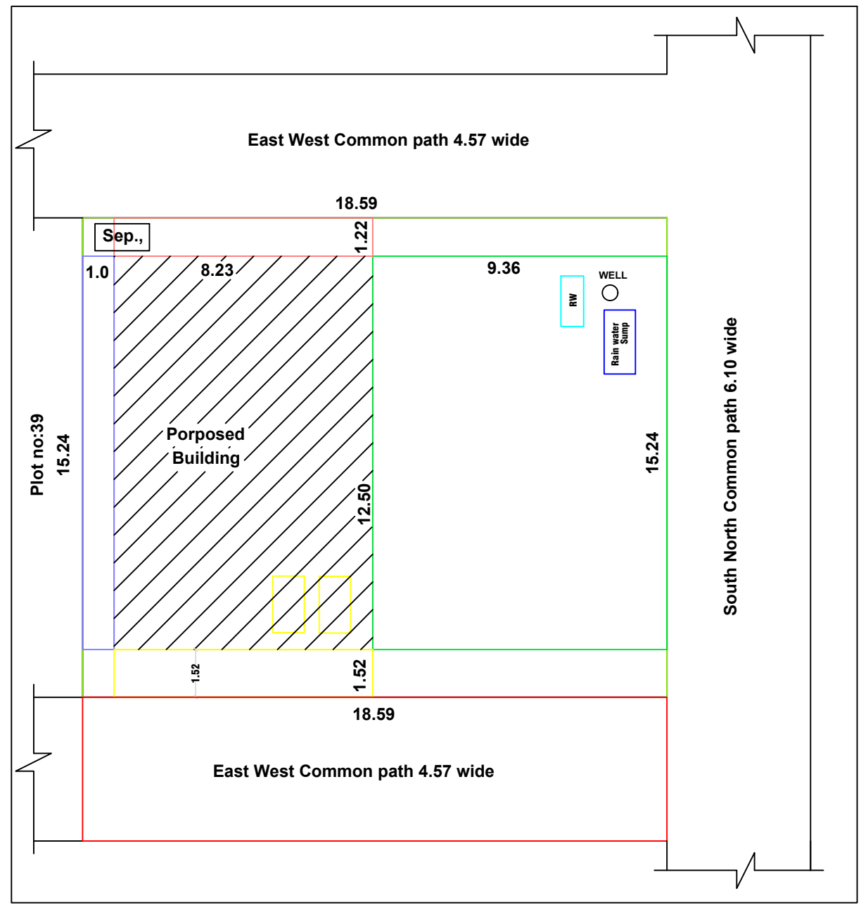
SITE PLAN CUM KEYPLAN
