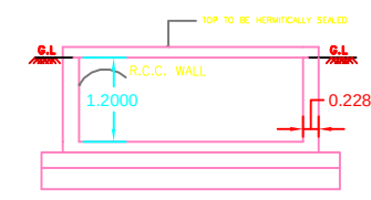
RWK SECTION (SAMPLE) RWK_CAPACITY_L=2000LTRS
