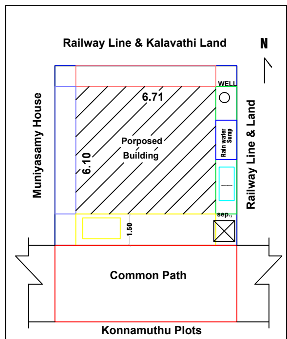
SITE PLAN CUM KEYPLAN
