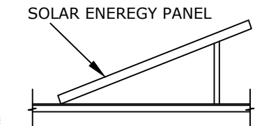
SYSTEM GENERAL POWER SCALE- N.T.S
