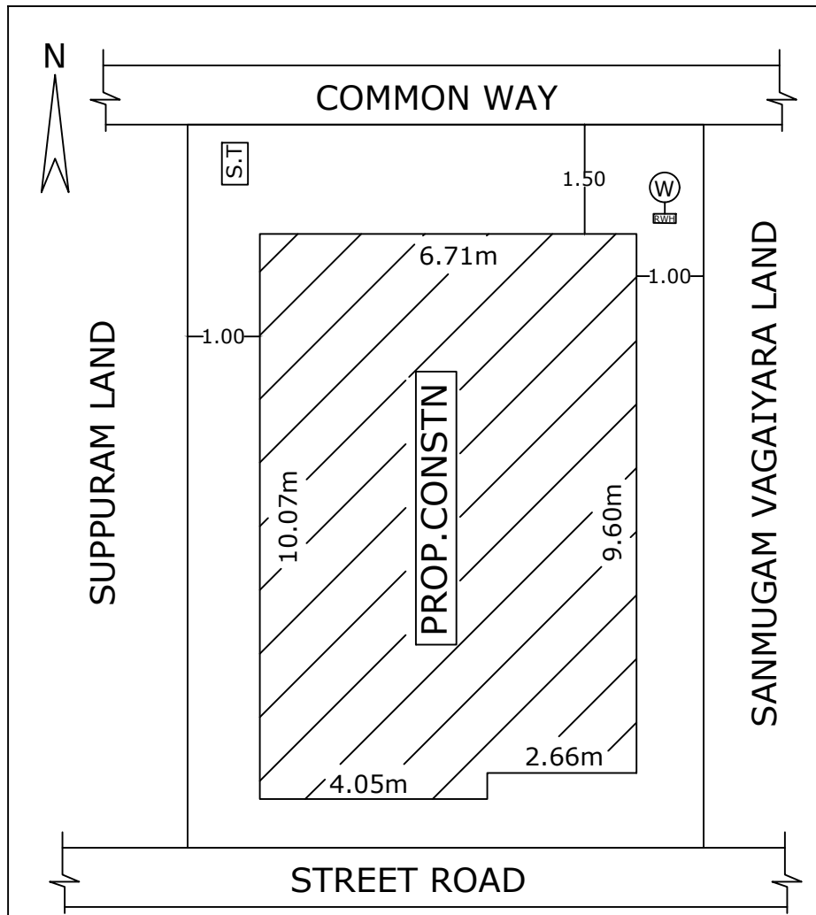
SITE PLAN
