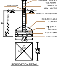
FOUNDATION DETAIL
