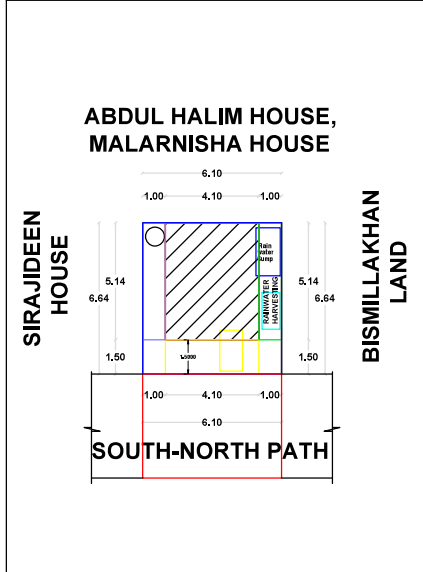
SITE PLAN & KEY PLAN (1:100)
