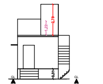
FRONT ELEVATION
