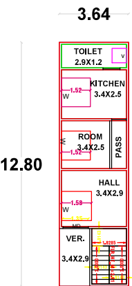
GROUND FLOOR I
