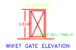
WIKET GATE ELEVATION
