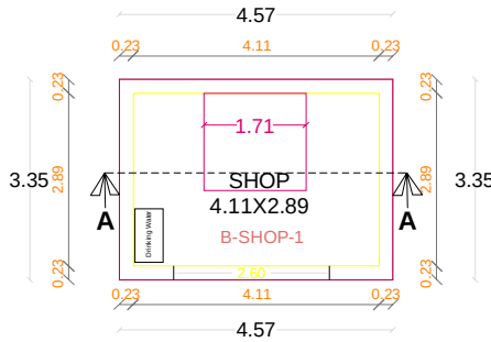
GROUND FLOOR PLAN PROPOSED
