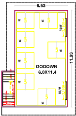
GROUND FLOOR PLAN
