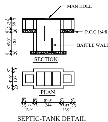
SEPTIC-TANK DETAIL
