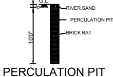
PERCULATION PIT
