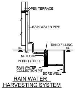
HARVESTING SYSTEM
