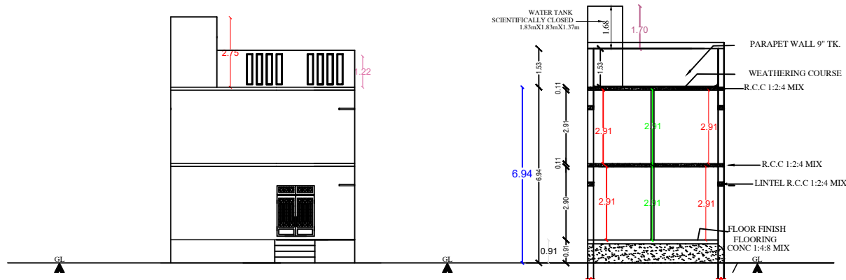
FRONT ELEVATION
