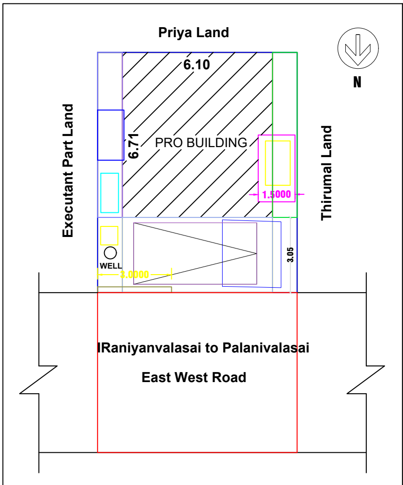
SITE PLAN
