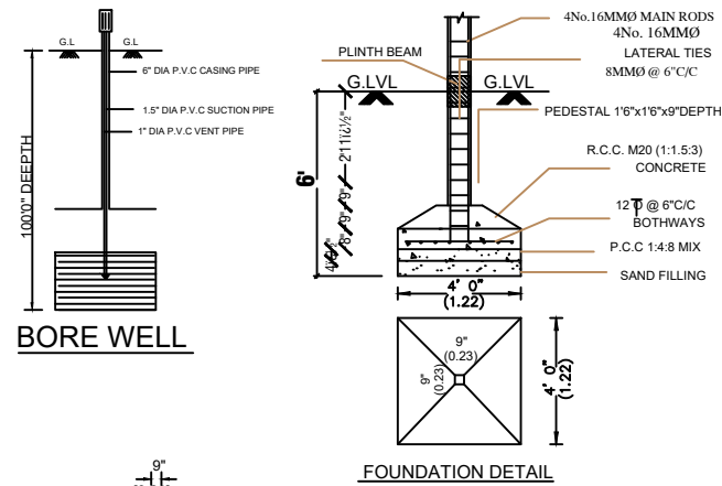
FOUNDATION DETAIL
