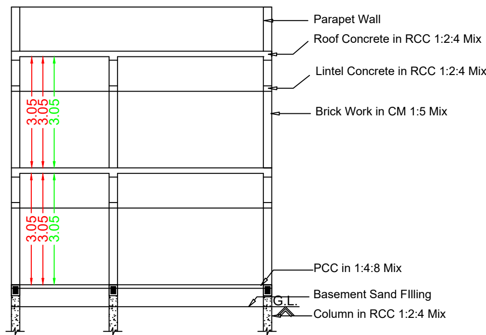
Section RR
