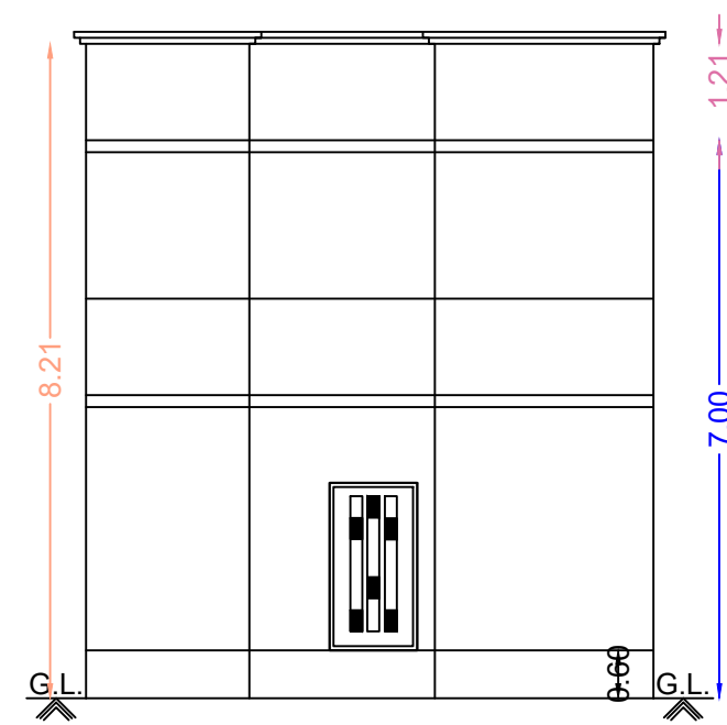
Front Elevation
