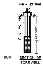
SECTION OF BORE WELL
