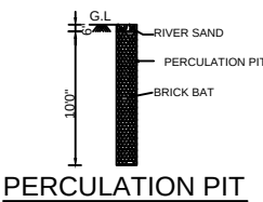
PERCOLATION PIT
