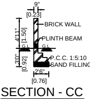
SECTION - CC
