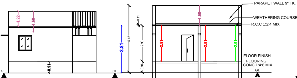
FRONT ELEVATION
