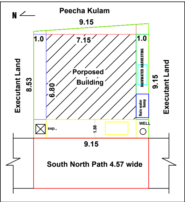
SITE PLAN CUM KEYPLAN
