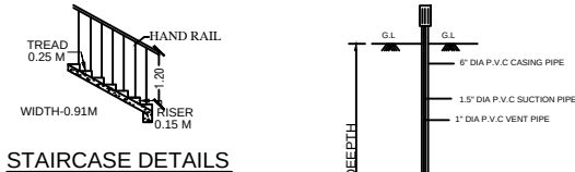
STAIRCASE DETAILS
