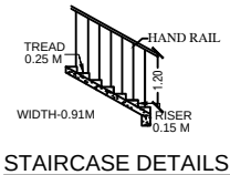
STAIRCASE DETAILS
