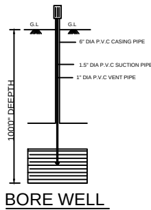
BORE WELL
