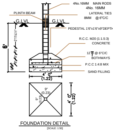
FOUNDATION DETAIL
