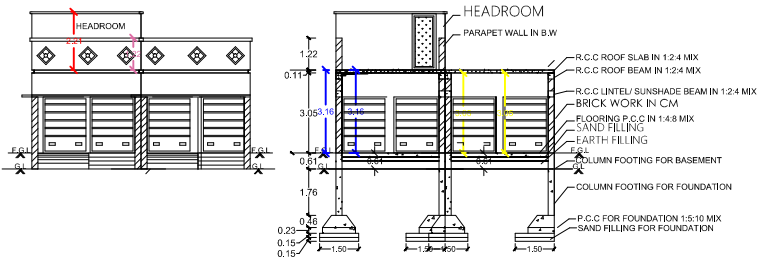
SECTION ON-A-A
