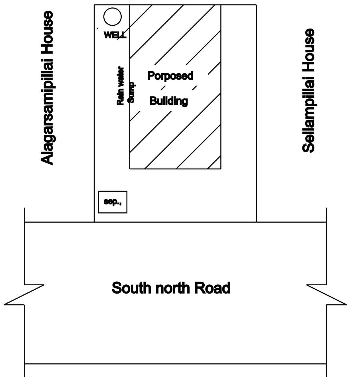
SITE PLAN CUM KEYPLAN
