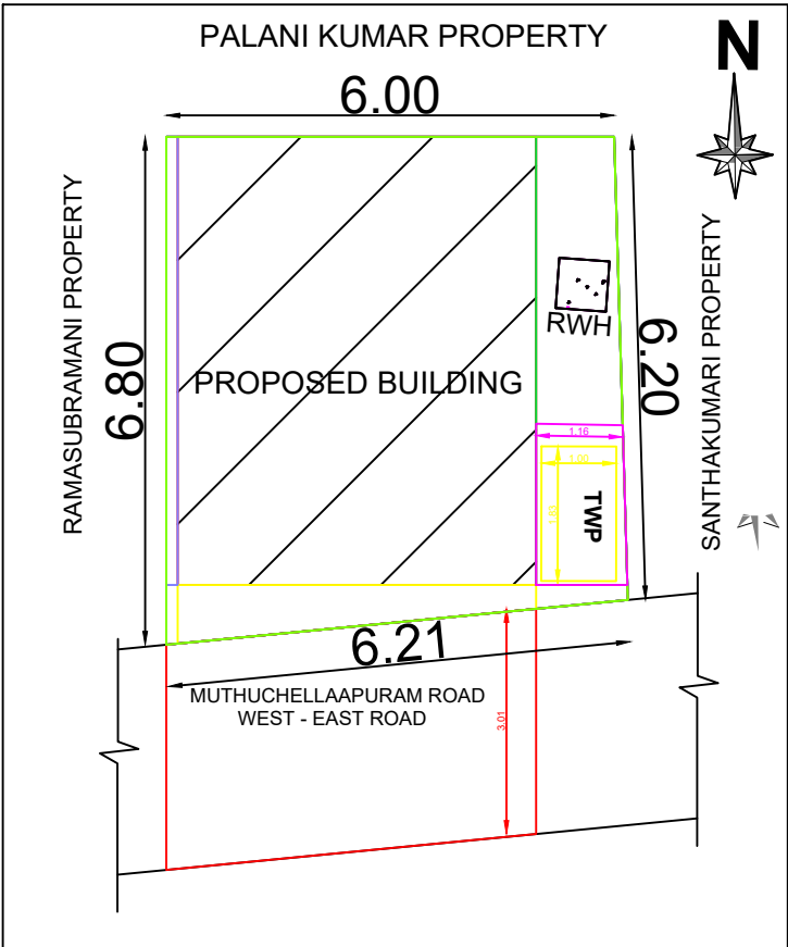
SITE PLAN
