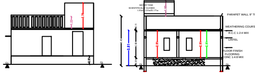
FRONT ELEVATION
