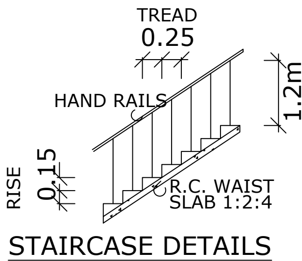
STAIRCASE DETAILS
