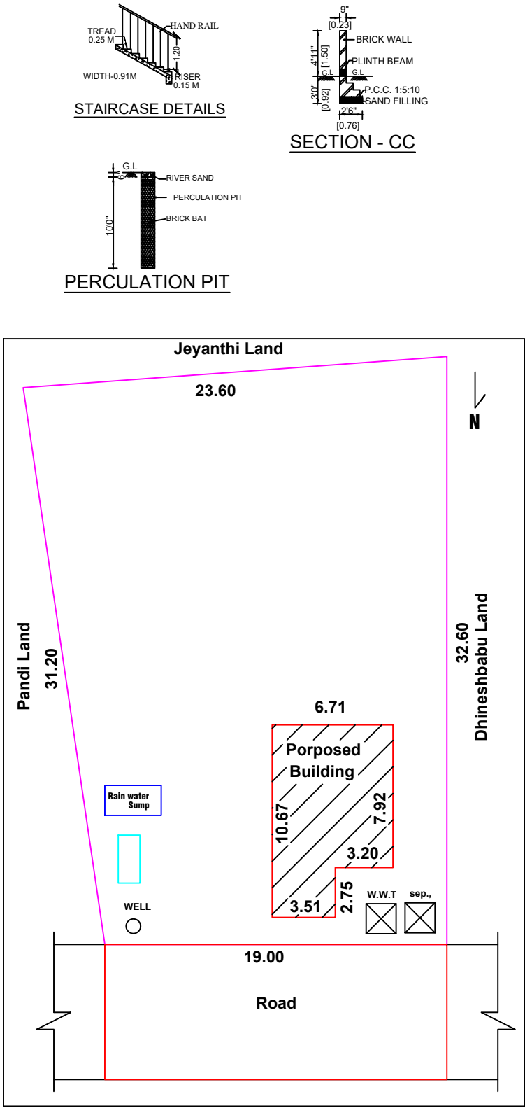
SITE PLAN CUM KEYPLAN
