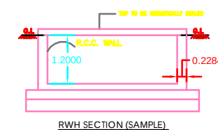
RWH_CAPACITY_L=2000LTRS
