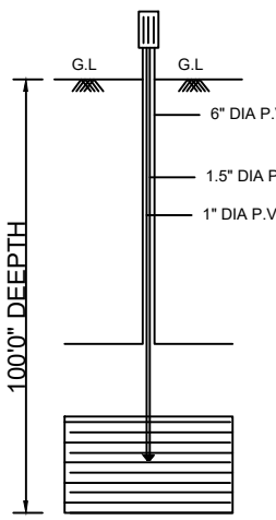
BORE WELL
