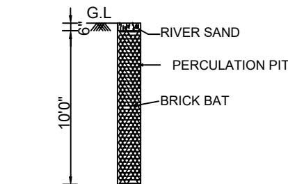
PERCULATION PIT
