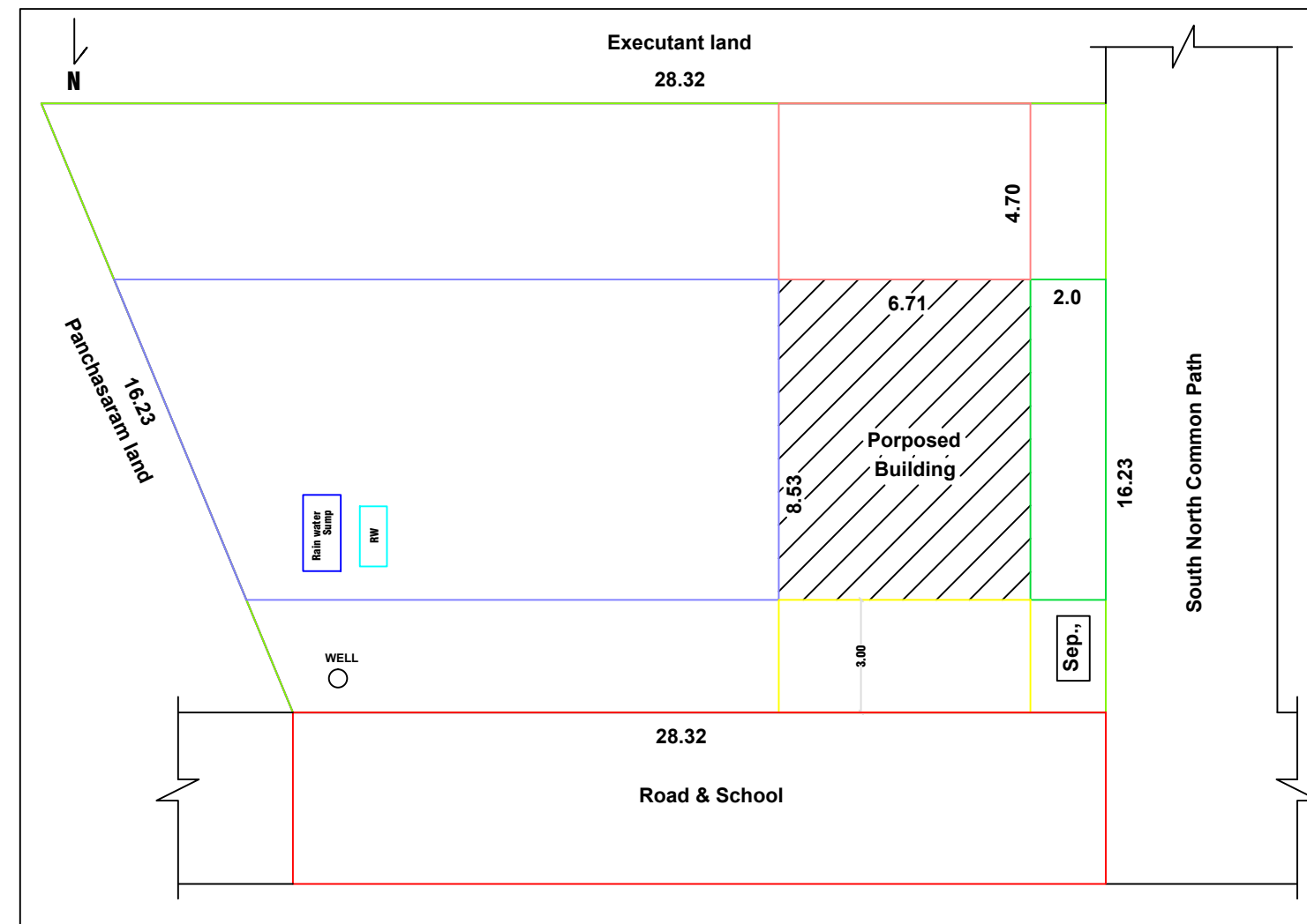
SITE PLAN CUM KEYPLAN
