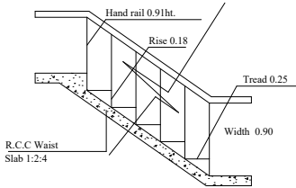
STAIRCASE DETAIL
