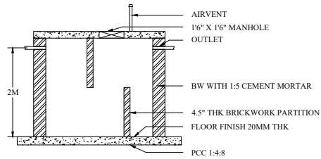
CROSS SECTION OF SEPTIC TANK
