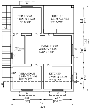
PROPOSED SECOND FLOOR PLAN
