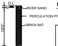
PERCOLATION PIT
