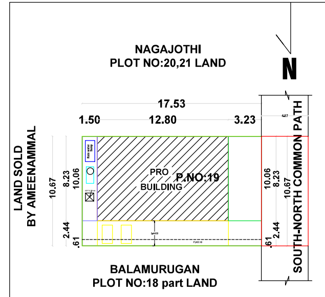
SITE PLAN & LOCATION PLAN
