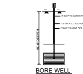
BORE WELL
