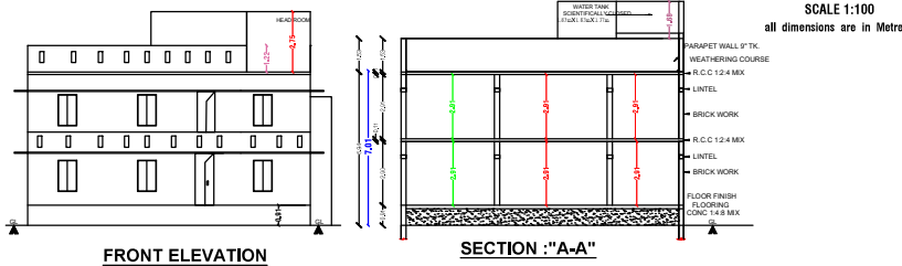
FRONT ELEVATION
