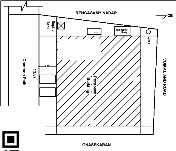
SITE PLAN CUM KEY PLAN
