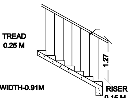
STAIRCASE DETAILS
