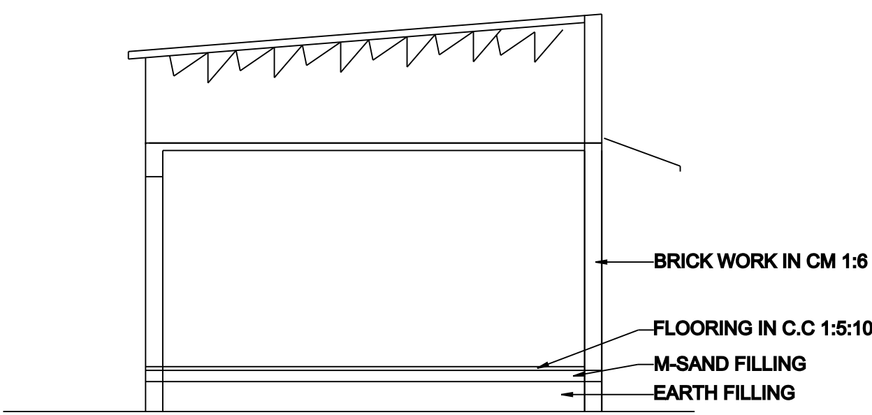
SECTION
