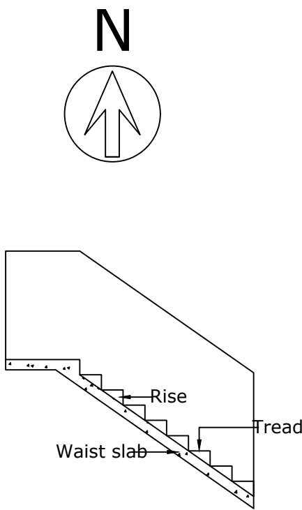
DETAILS OF STAIR CASE
