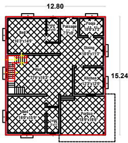
EXISTING GROUND FLOOR PLAN
