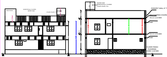
FRONT ELEVATION
