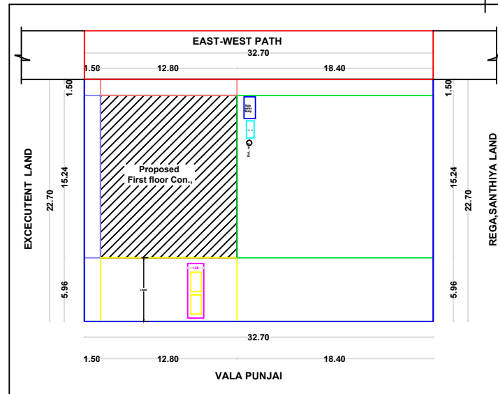
SITE PLAN & KEY PLAN (1:100)
