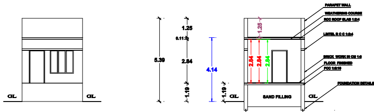
FRONT ELEVATION
