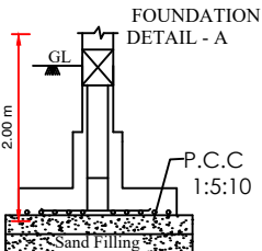
Isolated Footing -A (1.50X1.50) (Not to Scale)
