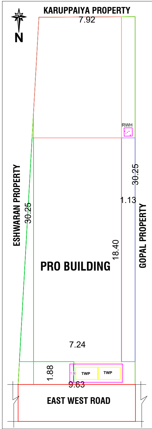
SITE PLAN
