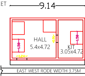
SITE PLAN CUM GROUND FLOOR PLAN
