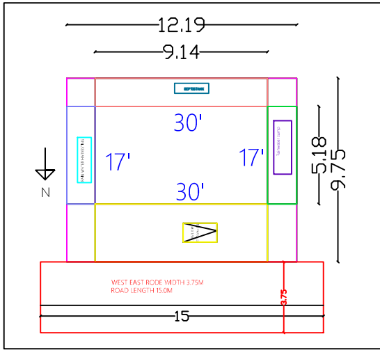
SITE PLAN CUM GROUND FLOOR PLAN
