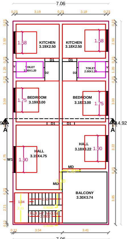
FIRST FLOOR PLAN PROPOSED
