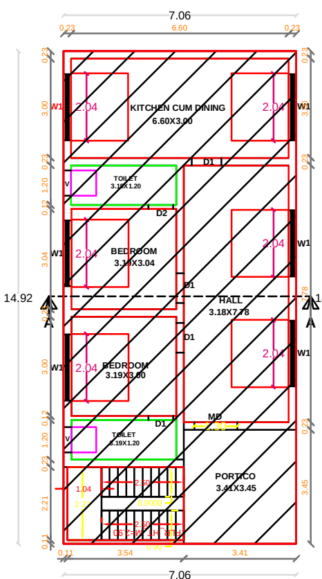
GROUND FLOOR PLAN EXISTING
