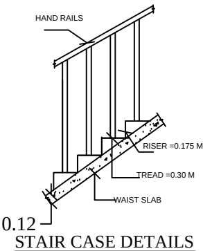
STAIR CASE DETAILS
