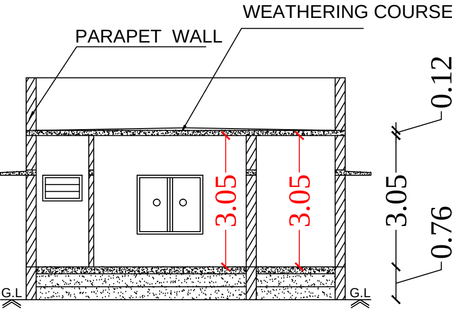
Section on-"AA"
