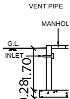
SECTION
